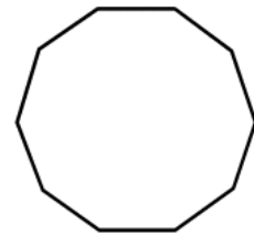
Regular Decagon
