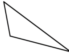
Scalene Triangle
