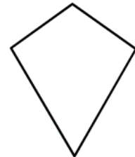
Kite
