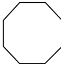
Regular Octagon
