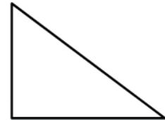
Right Triangle
